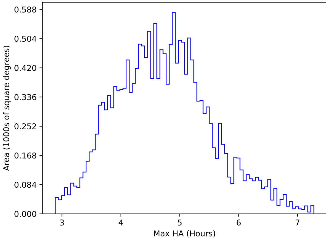
weather_cloudso0v3.5_10yrs WFD r band: Max HA
