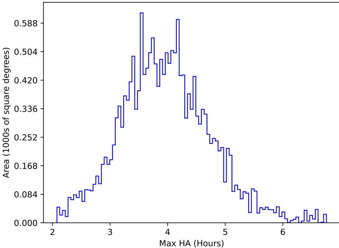
weather_cloudso0v3.5_10yrs WFD g band: Max HA
