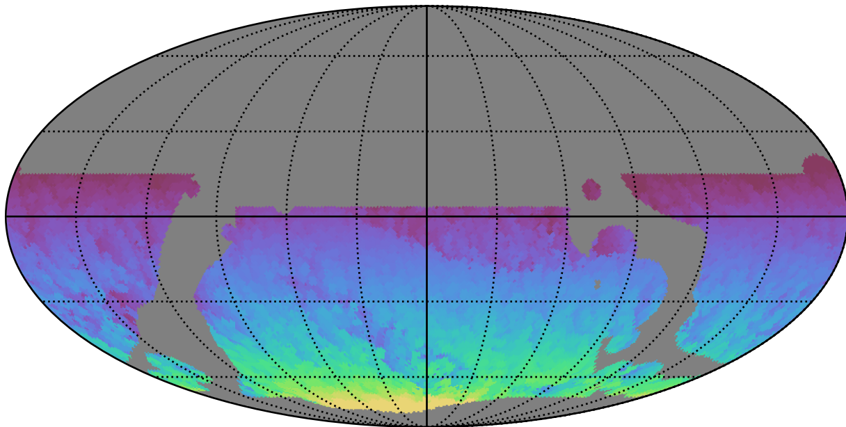
weather_cloudso0v3.5_10yrs WFD all bands: Max HA
