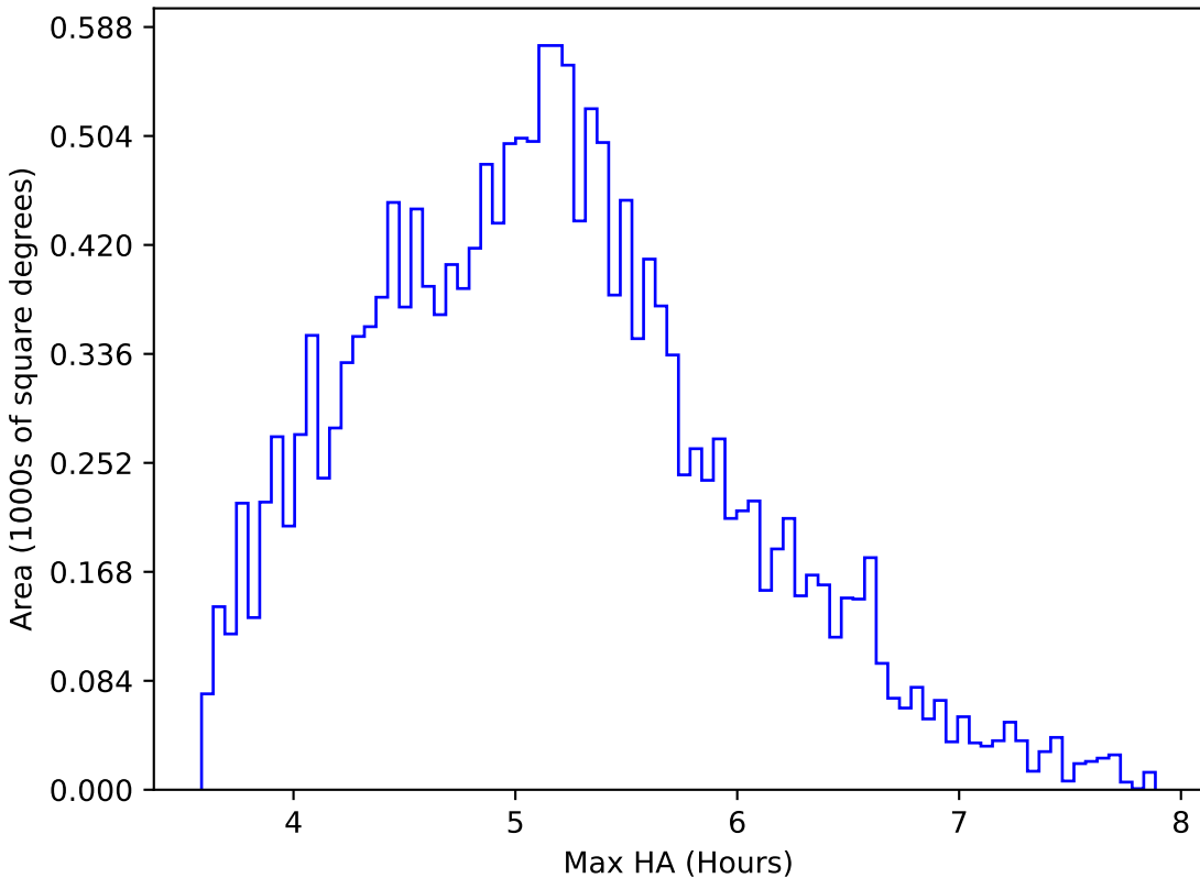
weather_cloudso0v3.5_10yrs WFD all bands: Max HA
