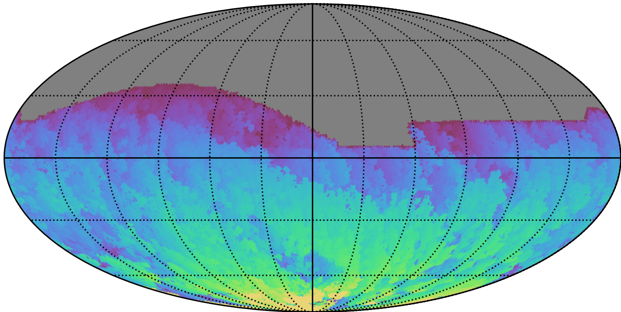
weather_cloudso0v3.5_10yrs All sky z band: Max HA
