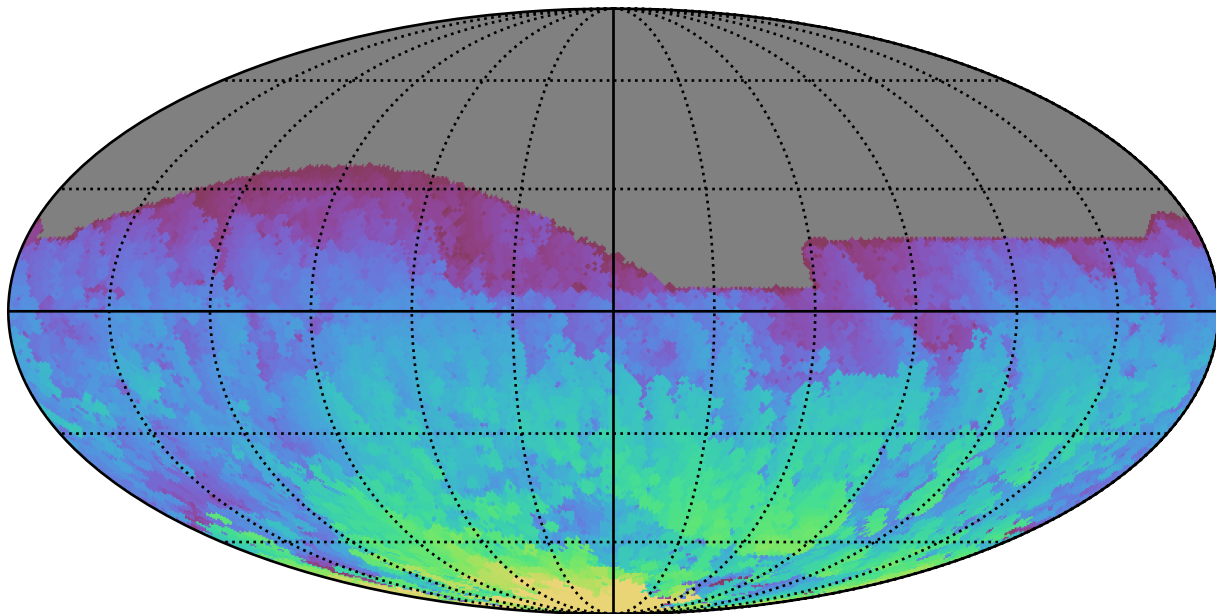
weather_cloudso0v3.5_10yrs All sky r band: Max HA
