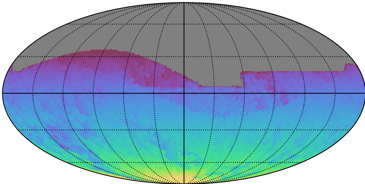
weather_cloudso0v3.5_10yrs All sky all bands: Max HA
