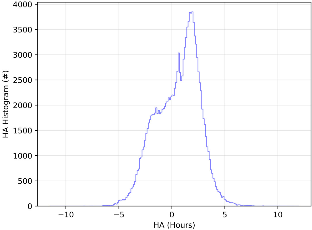
weather_cloudso0v3.5_10yrs WFD u band: HA Histogram
