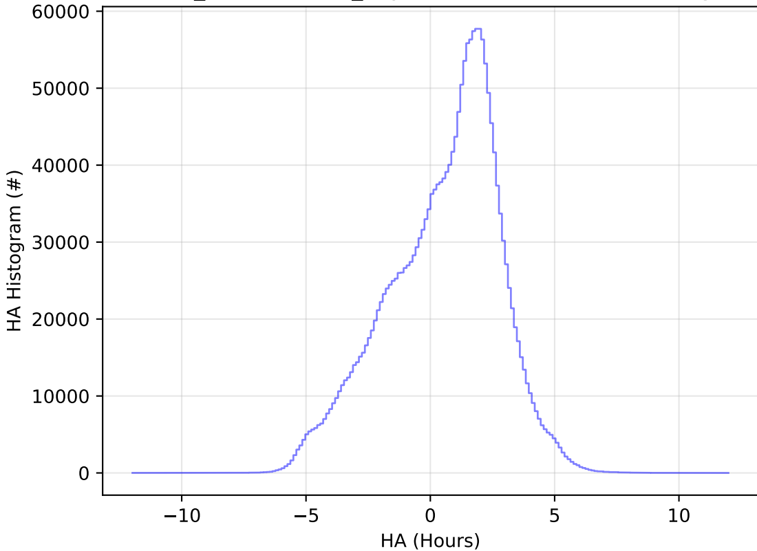
weather_cloudso0v3.5_10yrs WFD all bands: HA Histogram
