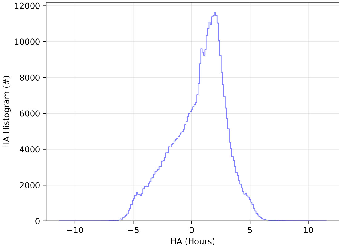
weather_cloudso0v3.5_10yrs All sky z band: HA Histogram
