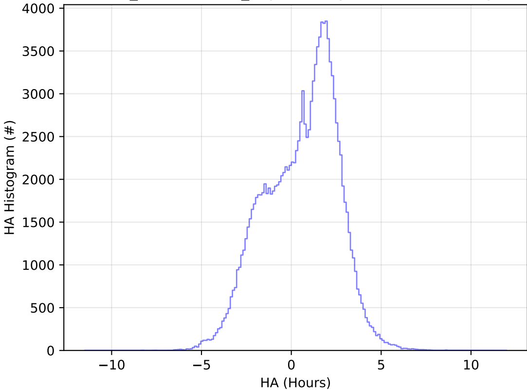
weather_cloudso0v3.5_10yrs All sky u band: HA Histogram
