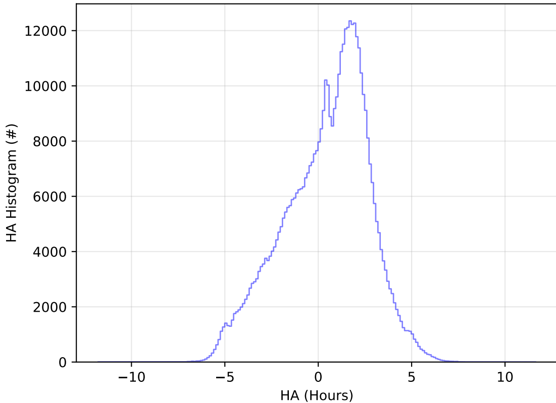
weather_cloudso0v3.5_10yrs All sky r band: HA Histogram
