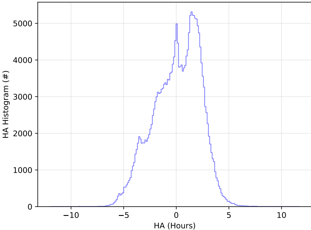
weather_cloudso0v3.5_10yrs All sky g band: HA Histogram
