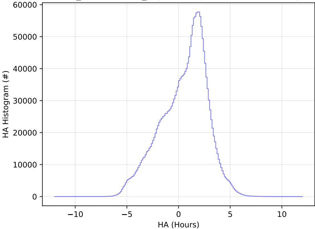
weather_cloudso0v3.5_10yrs All sky all bands: HA Histogram
