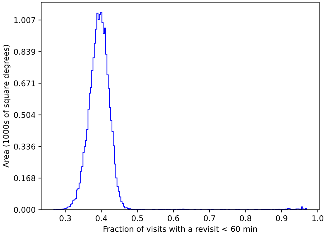
weather_cloudso0v3.5_10yrs gri WFD: Fraction of visits with a revisit < 60 min
