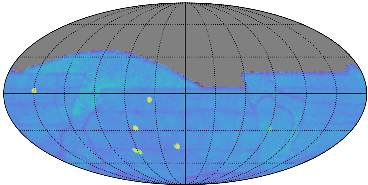
weather_cloudso0v3.5_10yrs gri All sky: Fraction of visits with a revisit < 60 min
