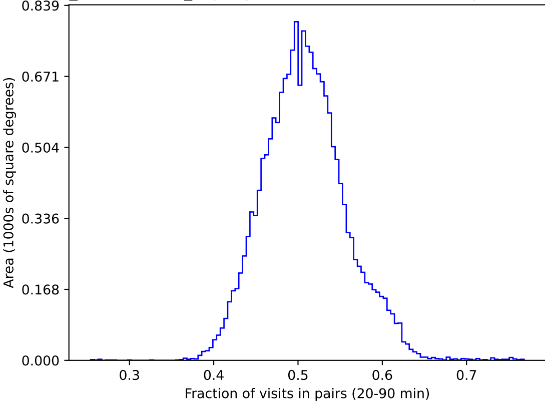
weather_cloudso0v3.5_10yrs gri WFD: Fraction of visits in pairs (20-90 min)
