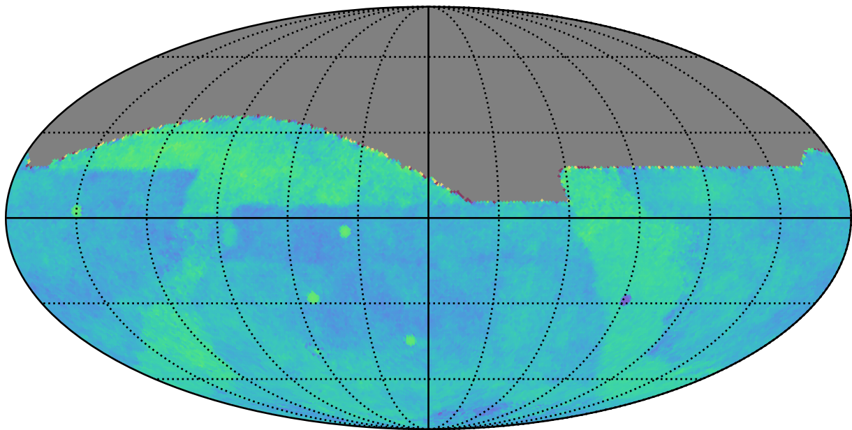
weather_cloudso0v3.5_10yrs gri All sky: Fraction of visits in pairs (20-90 min)
