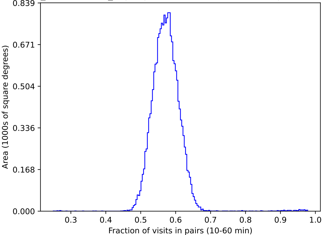
weather_cloudso0v3.5_10yrs gri WFD: Fraction of visits in pairs (10-60 min)
