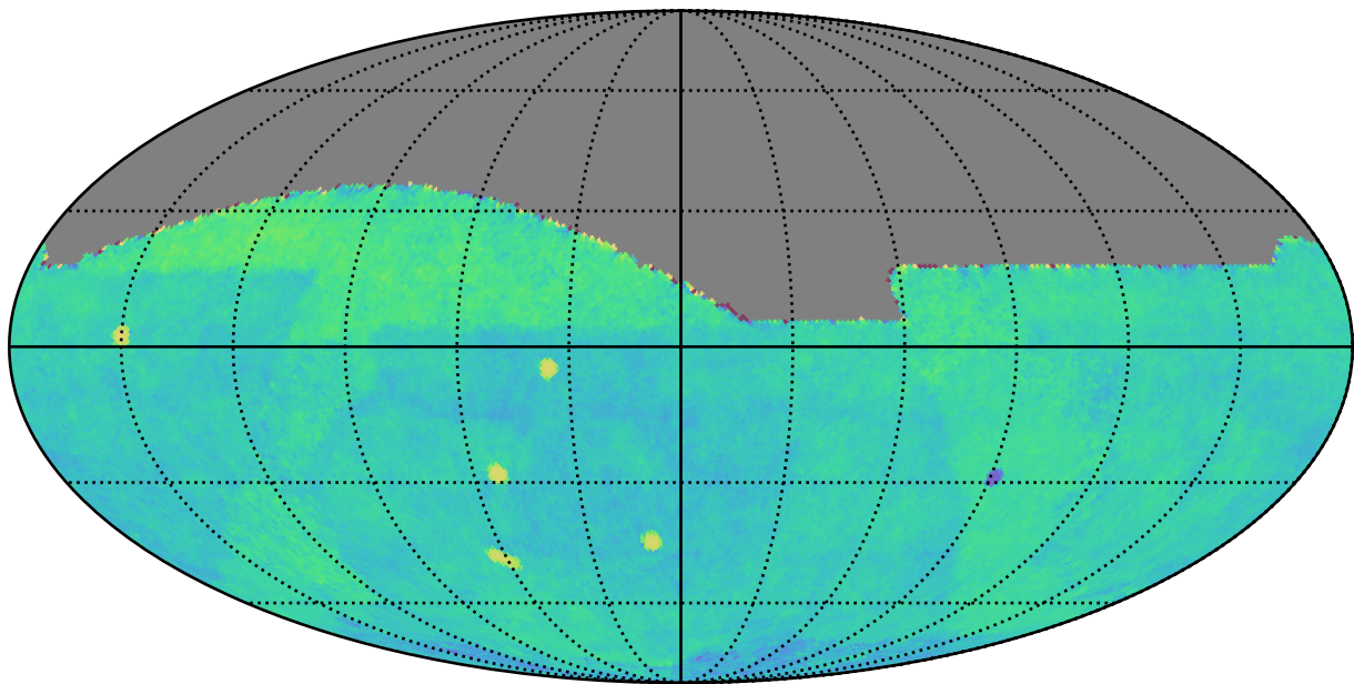
weather_cloudso0v3.5_10yrs gri All sky: Fraction of visits in pairs (10-60 min)
