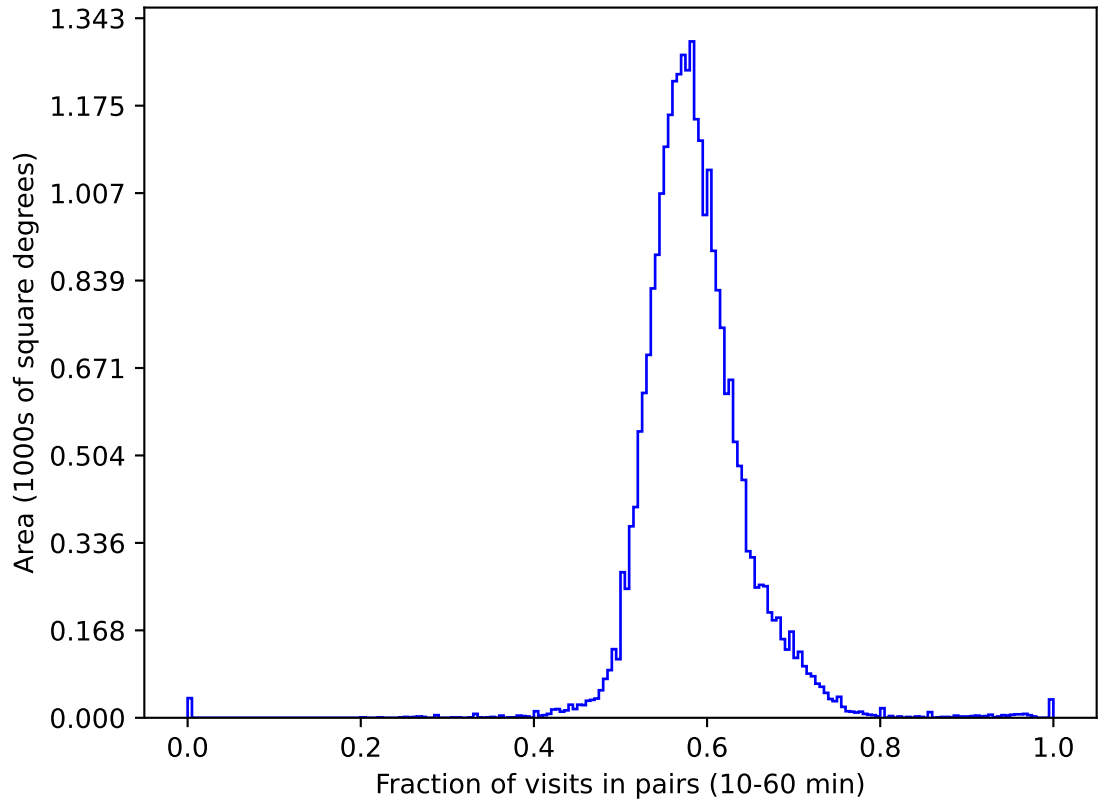
weather_cloudso0v3.5_10yrs gri All sky: Fraction of visits in pairs (10-60 min)
