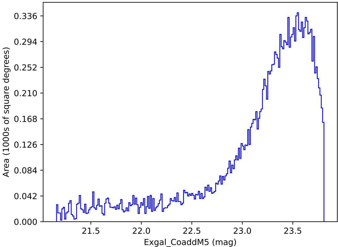
weather_cloudso0v3.5_10yrs Yr 3-4 y band: Exgal_CoaddM5
