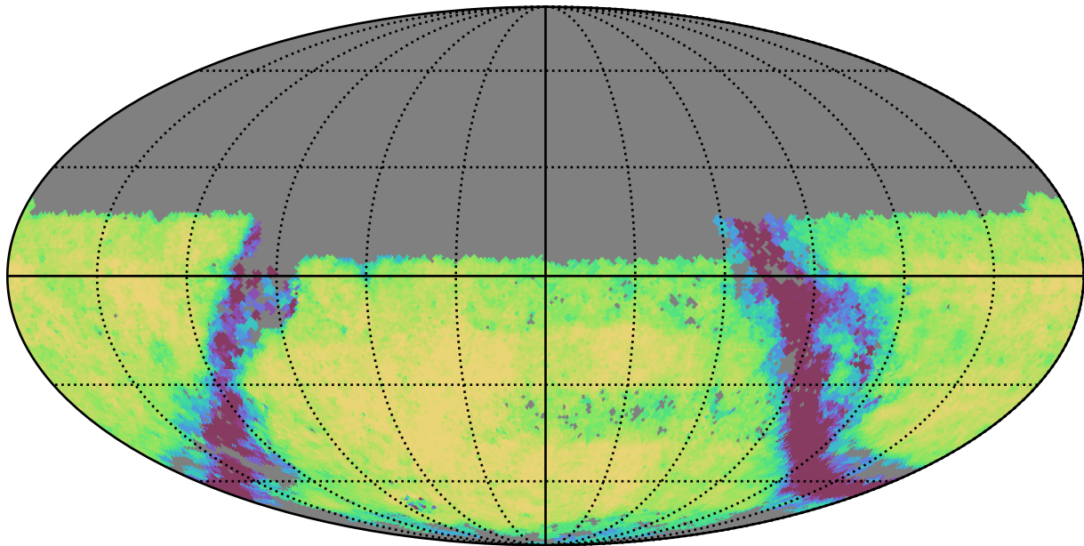
weather_cloudso0v3.5_10yrs Yr 3-4 u band: Exgal_CoaddM5
