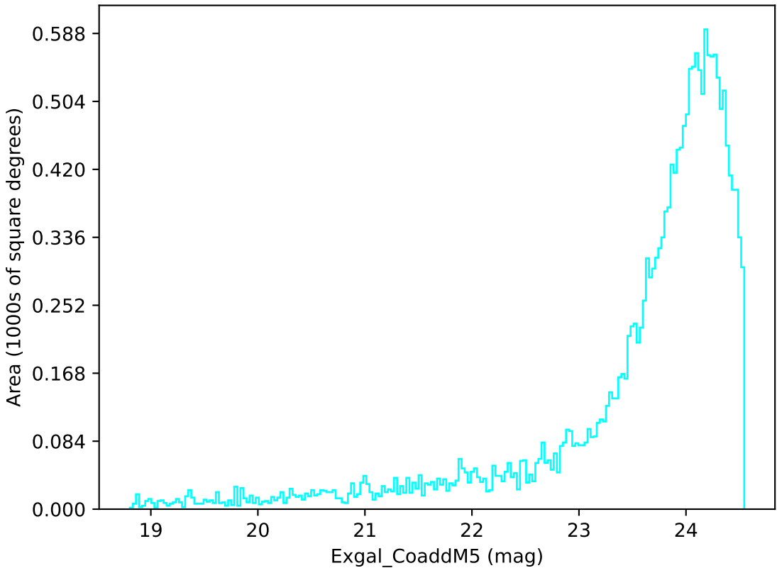
weather_cloudso0v3.5_10yrs Yr 3-4 u band: Exgal_CoaddM5
