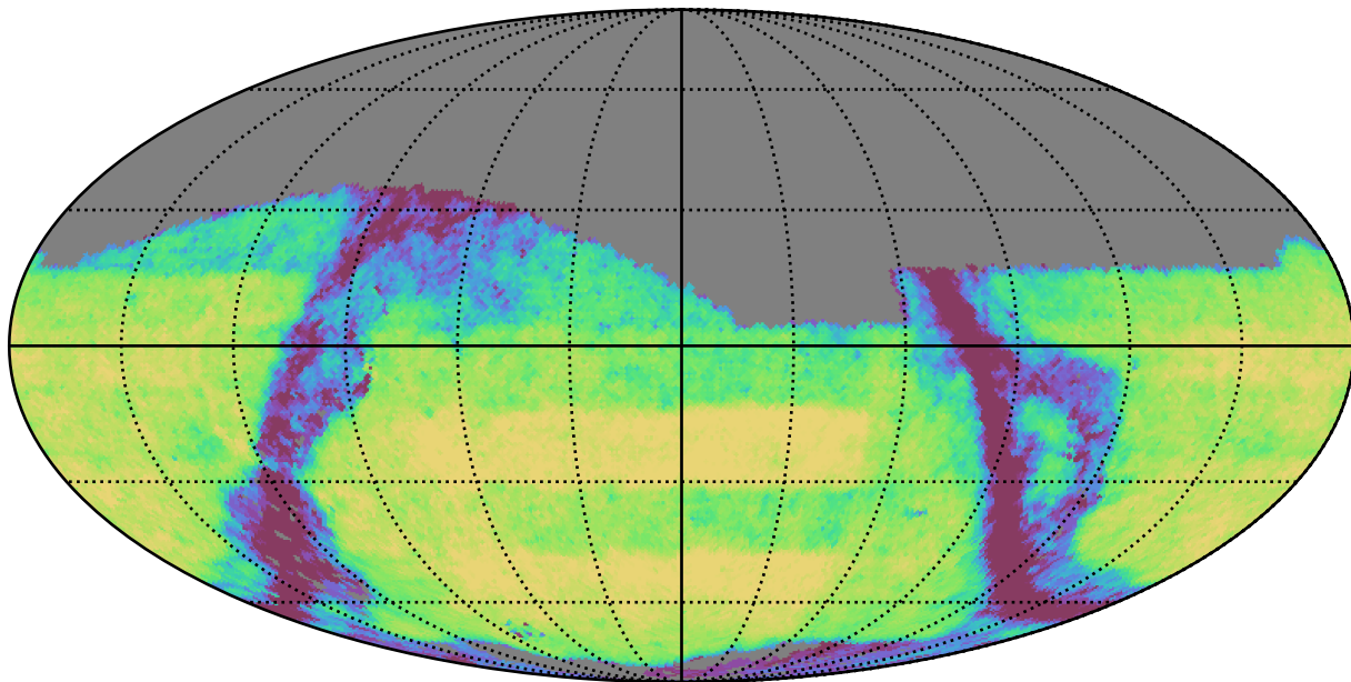
weather_cloudso0v3.5_10yrs Yr 3-4 i band: Exgal_CoaddM5
