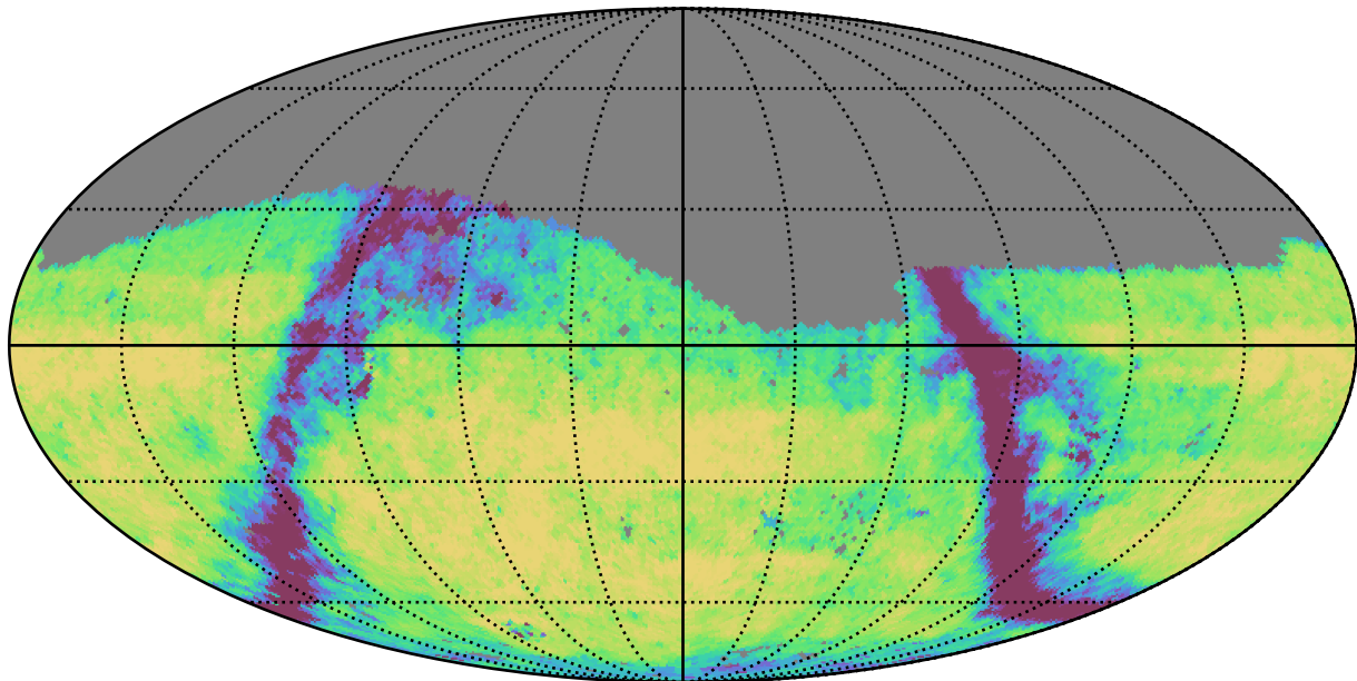
weather_cloudso0v3.5_10yrs Yr 3-4 g band: Exgal_CoaddM5
