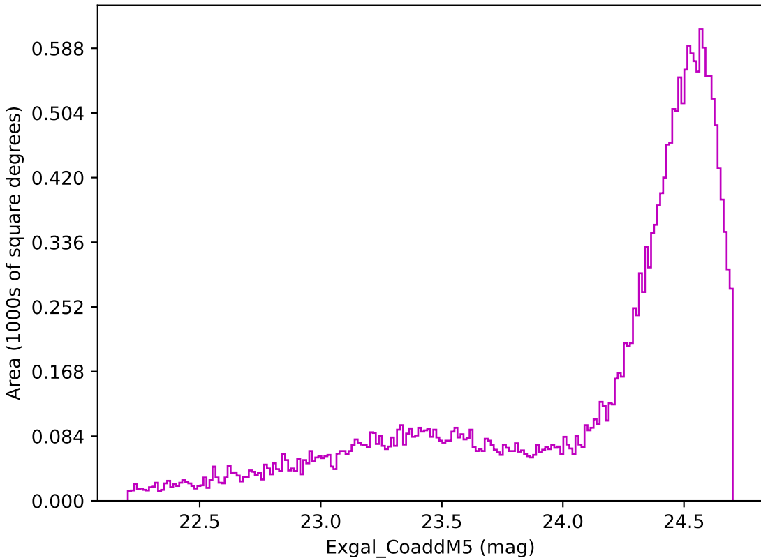
weather_cloudso0v3.5_10yrs Yr 1 z band: Exgal_CoaddM5
