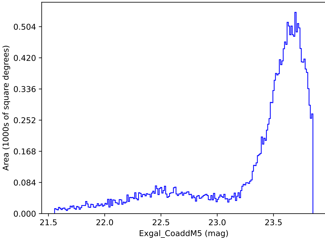
weather_cloudso0v3.5_10yrs Yr 1 y band: Exgal_CoaddM5
