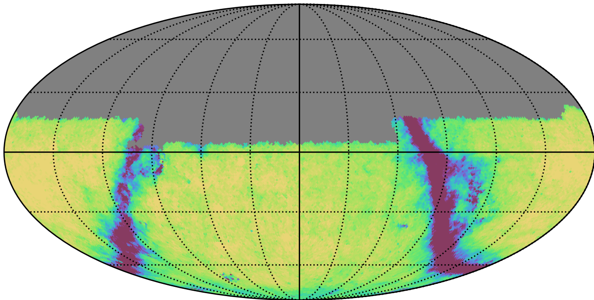
weather_cloudso0v3.5_10yrs Yr 1 u band: Exgal_CoaddM5
