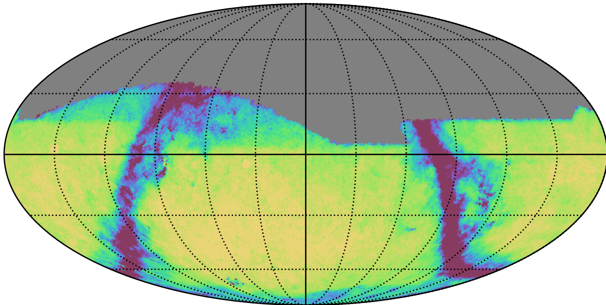
weather_cloudso0v3.5_10yrs Yr 1 r band: Exgal_CoaddM5
