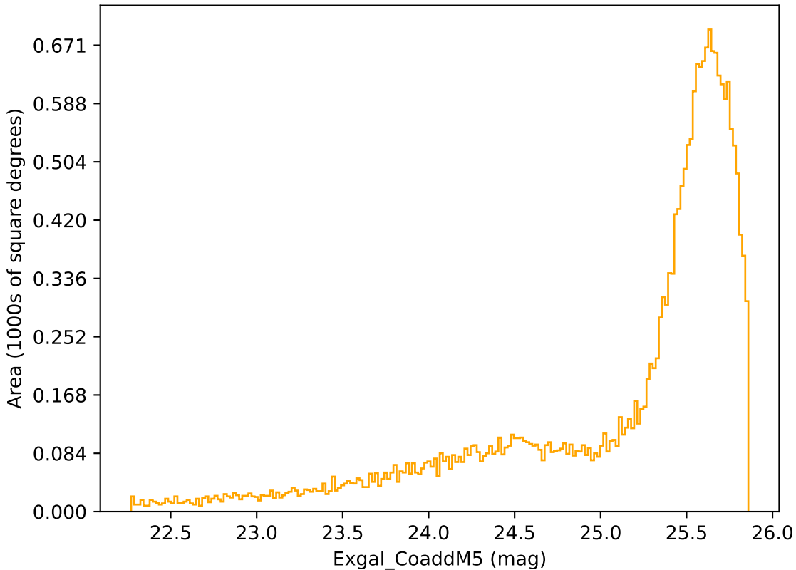
weather_cloudso0v3.5_10yrs Yr 1 r band: Exgal_CoaddM5
