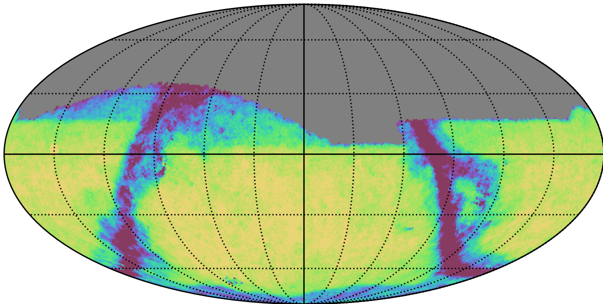
weather_cloudso0v3.5_10yrs Yr 1 i band: Exgal_CoaddM5
