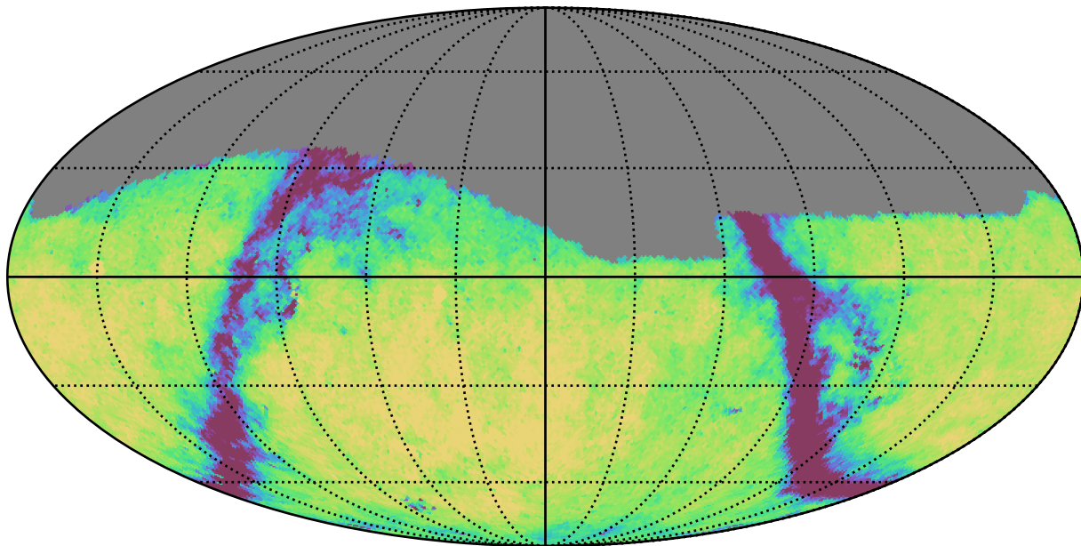
weather_cloudso0v3.5_10yrs Yr 1 g band: Exgal_CoaddM5
