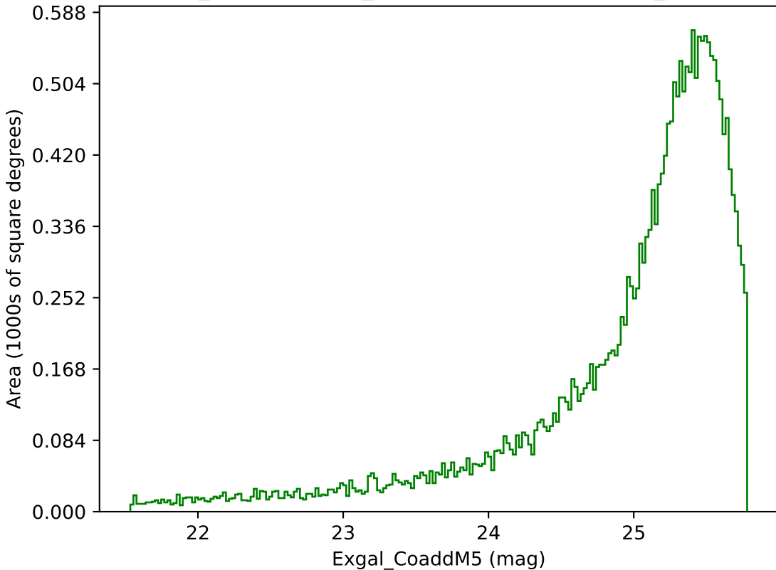
weather_cloudso0v3.5_10yrs Yr 1 g band: Exgal_CoaddM5
