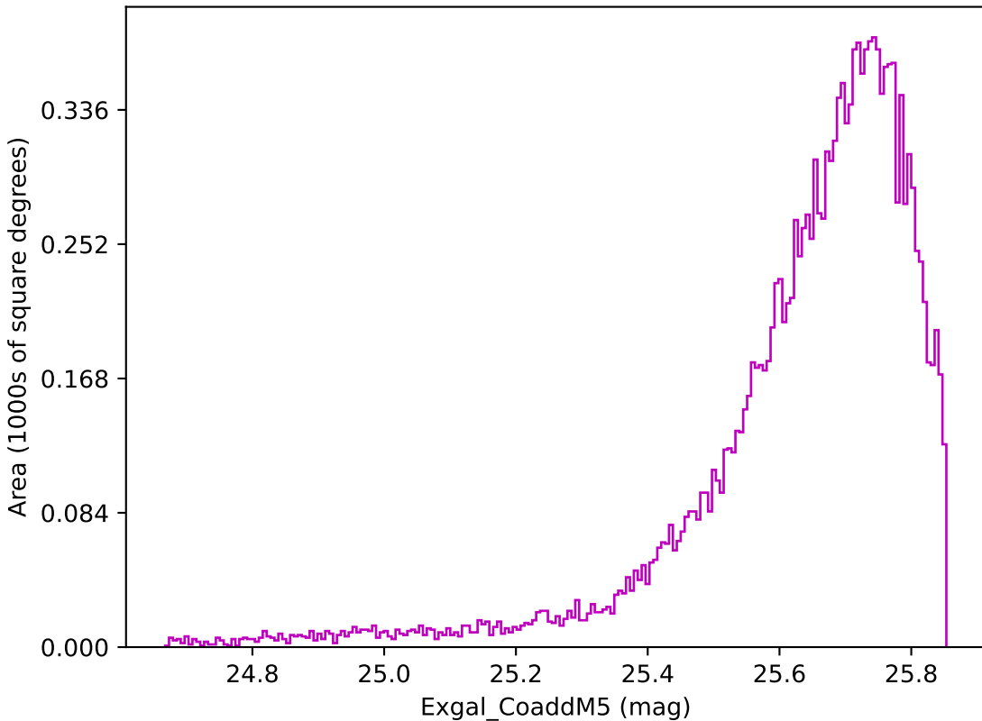
weather_cloudso0v3.5_10yrs WFD z band: Exgal_CoaddM5
