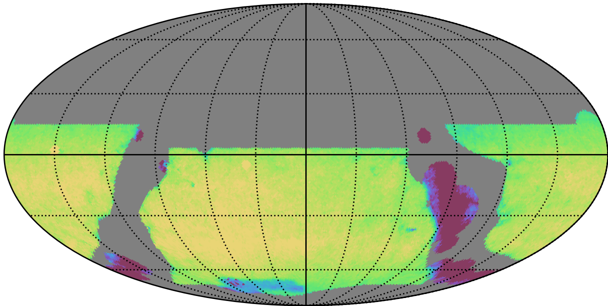
weather_cloudso0v3.5_10yrs WFD y band: Exgal_CoaddM5
