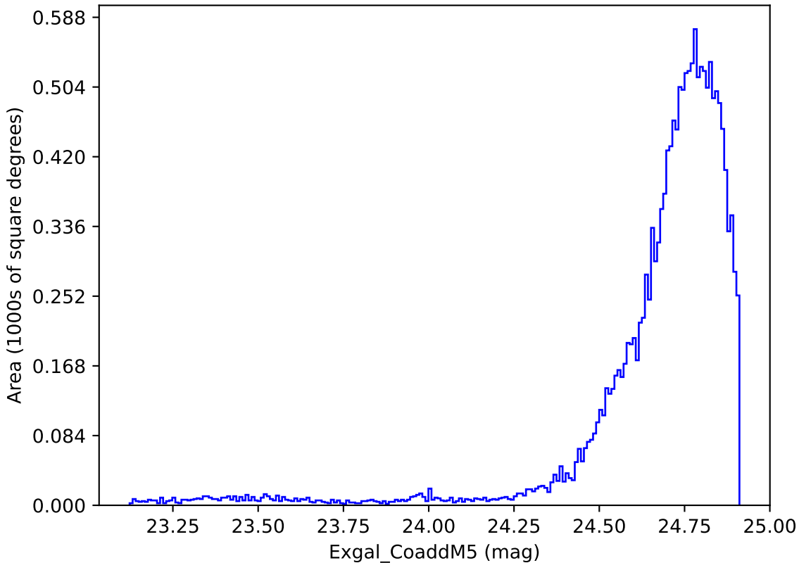
weather_cloudso0v3.5_10yrs WFD y band: Exgal_CoaddM5
