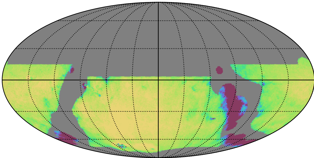
weather_cloudso0v3.5_10yrs WFD u band: Exgal_CoaddM5
