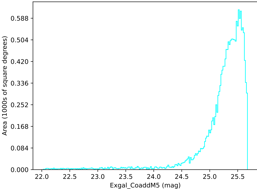
weather_cloudso0v3.5_10yrs WFD u band: Exgal_CoaddM5
