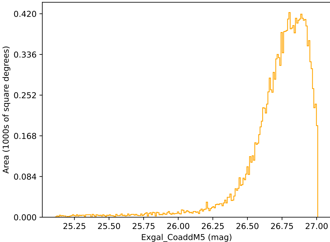
weather_cloudso0v3.5_10yrs WFD r band: Exgal_CoaddM5
