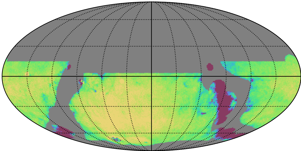
weather_cloudso0v3.5_10yrs WFD g band: Exgal_CoaddM5
