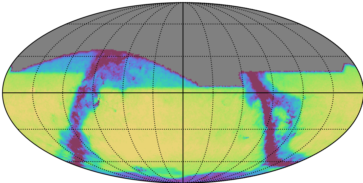
weather_cloudso0v3.5_10yrs All sky z band: Exgal_CoaddM5
