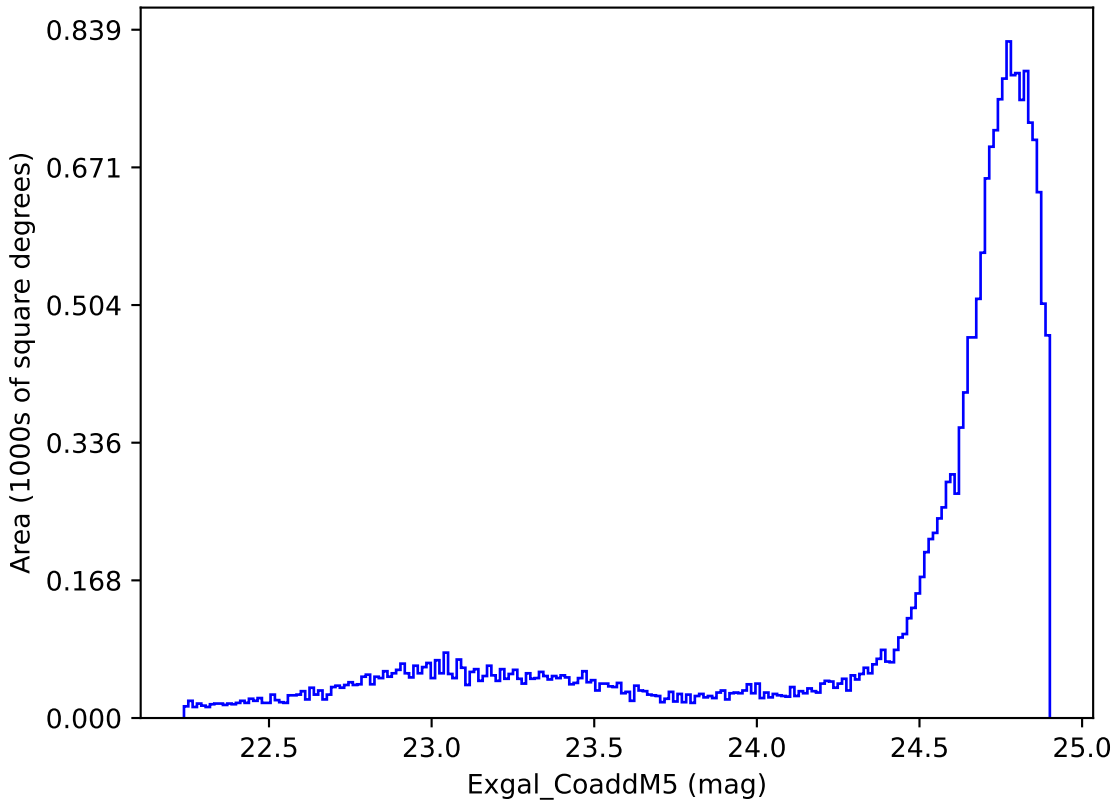
weather_cloudso0v3.5_10yrs All sky y band: Exgal_CoaddM5
