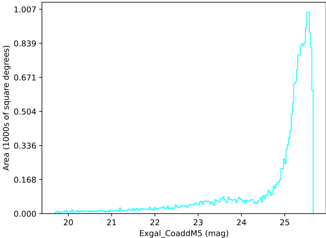
weather_cloudso0v3.5_10yrs All sky u band: Exgal_CoaddM5
