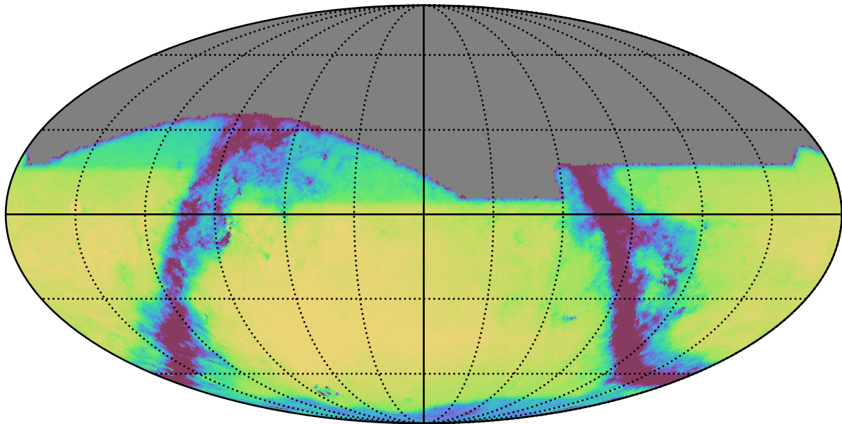
weather_cloudso0v3.5_10yrs All sky r band: Exgal_CoaddM5
