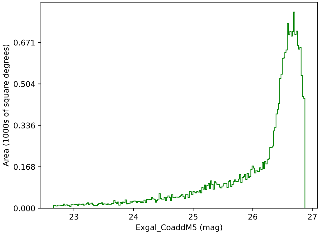
weather_cloudso0v3.5_10yrs All sky g band: Exgal_CoaddM5
