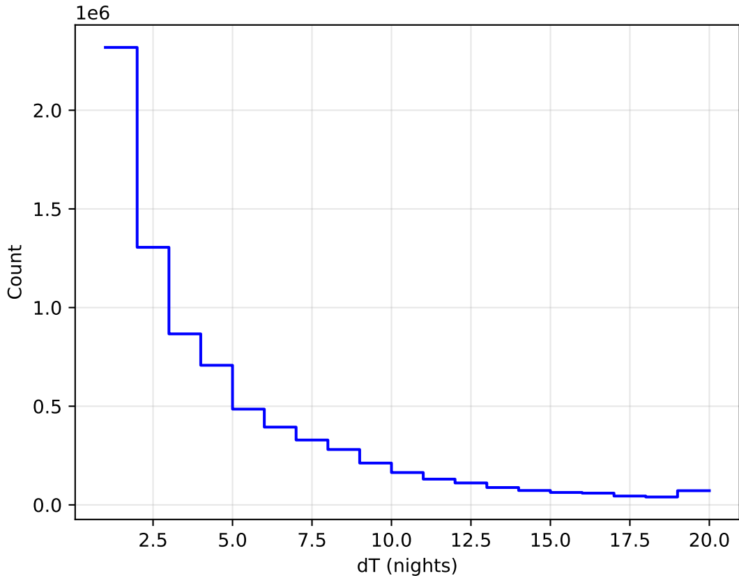
weather_cloudso0v3.5_10yrs WFD all bands: DeltaNight Histogram
