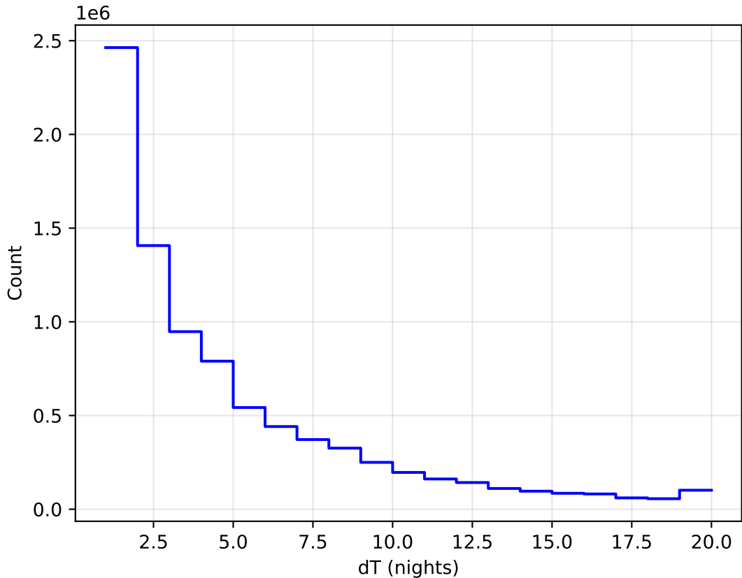
weather_cloudso0v3.5_10yrs All sky all bands: DeltaNight Histogram
