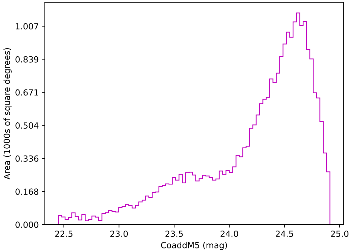
weather_cloudso0v3.5_10yrs Yr 3-4 z band: CoaddM5
