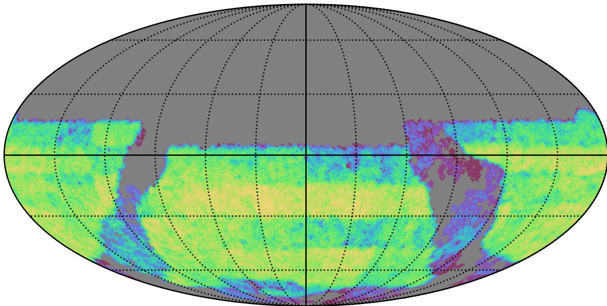
weather_cloudso0v3.5_10yrs Yr 3-4 y band: CoaddM5
